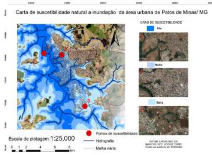
Figure 20: Chart of natural susceptibility to flooding in the urban area of Patos de Minas, Minas General.
